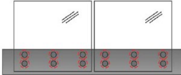
FIG. 8 Type VI: Point Supported Only—Glazing as Structural Member
